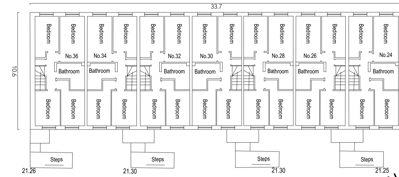
SECOND FLOOR
