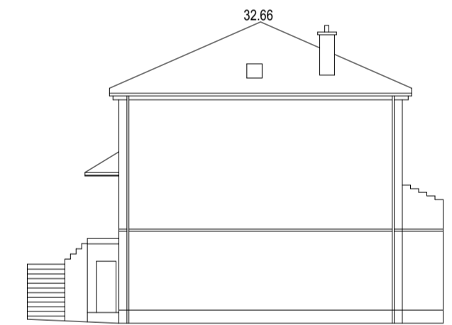
Datum 15.00 AOD Block B South Elevation
