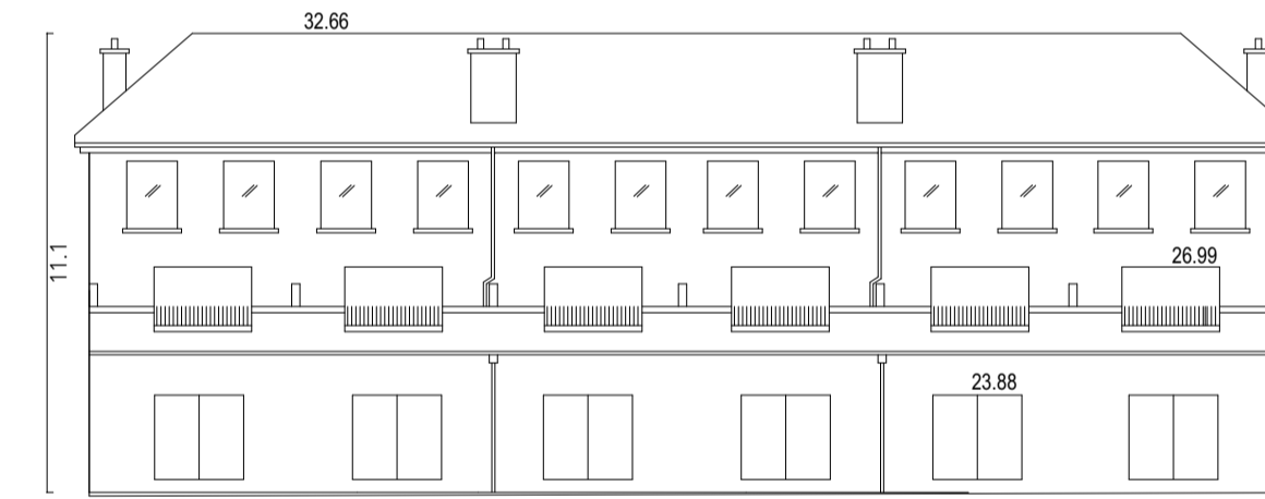
Datum 15.00 AOD Block B East Elevation
