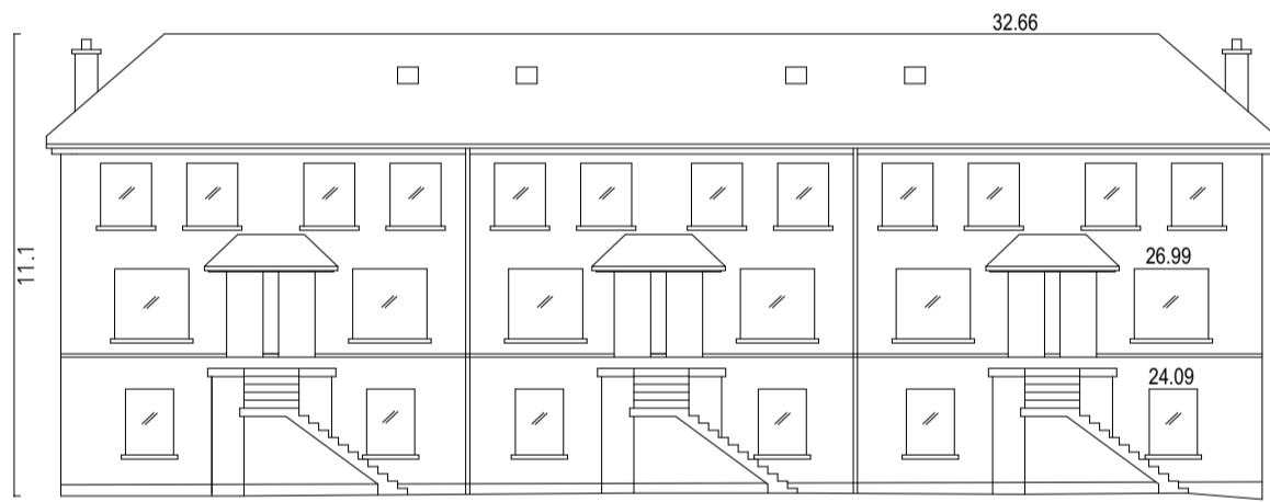
Datum 15.00 AOD Block B West Elevation
