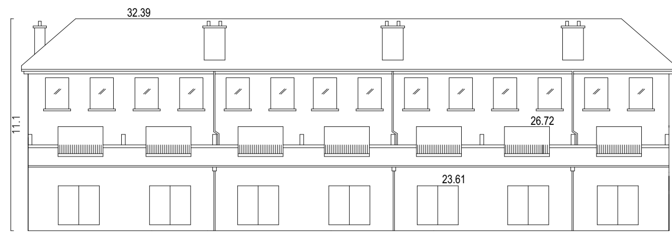
Datum 15.00 AOD Block A North Elevation
