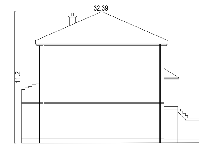
Datum 15.00 AOD Block A West Elevation
