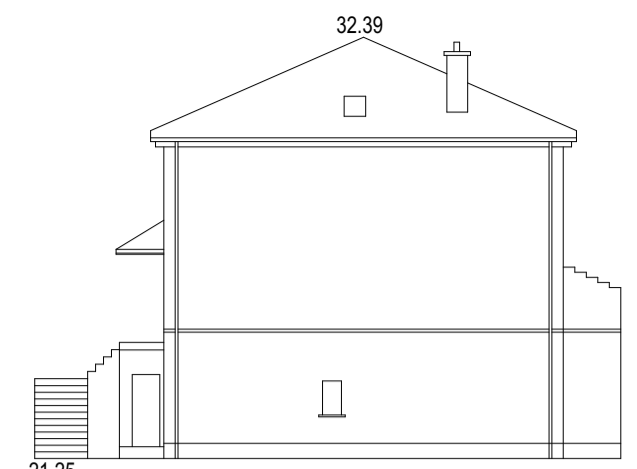
Datum 15.00 AOD Block A East Elevation
