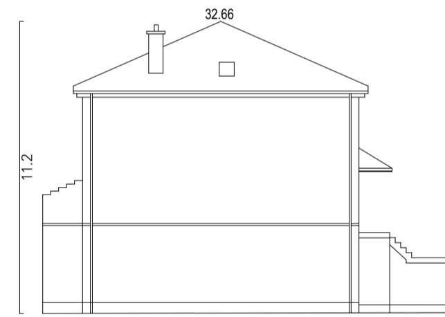
Datum 15.00 AOD Block B North Elevation
