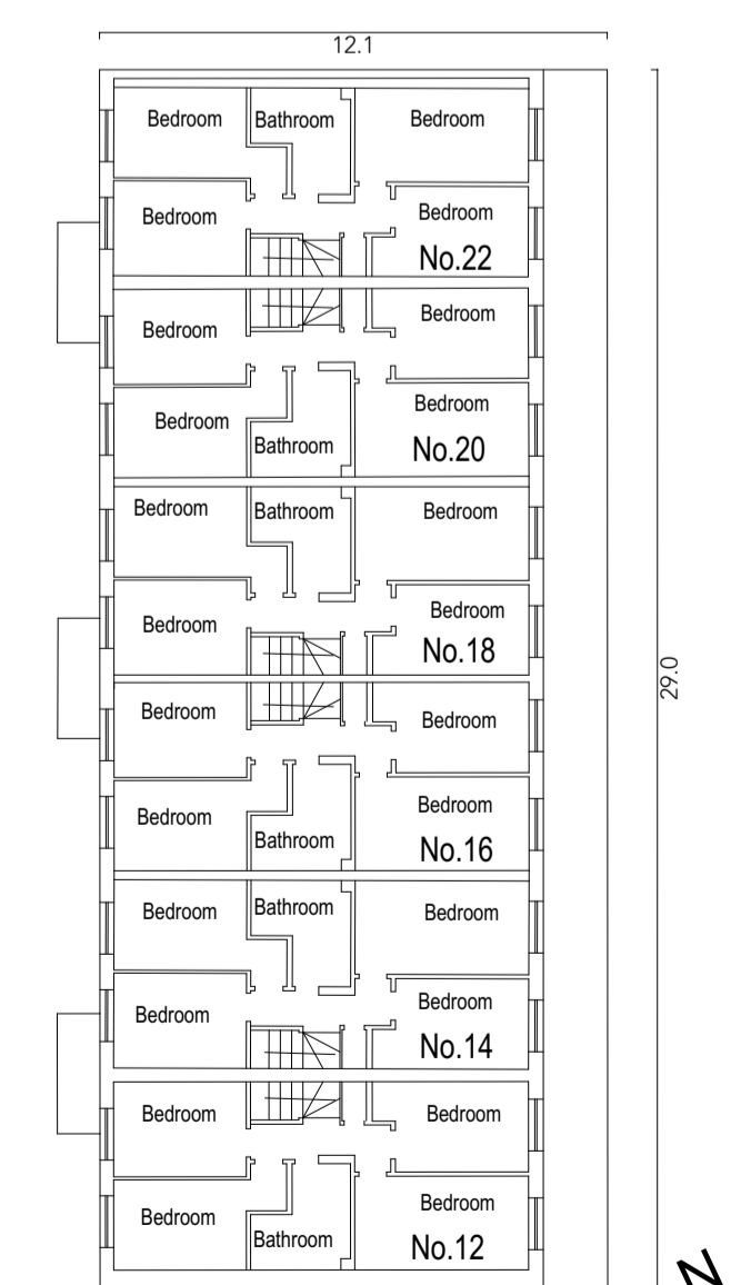
SECOND FLOOR
