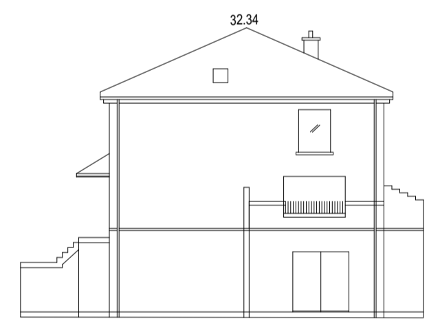
Datum 15.00 AOD Block D South Elevation
