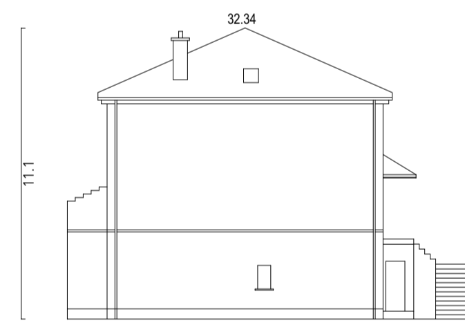
Datum 15.00 AOD Block D North Elevation
