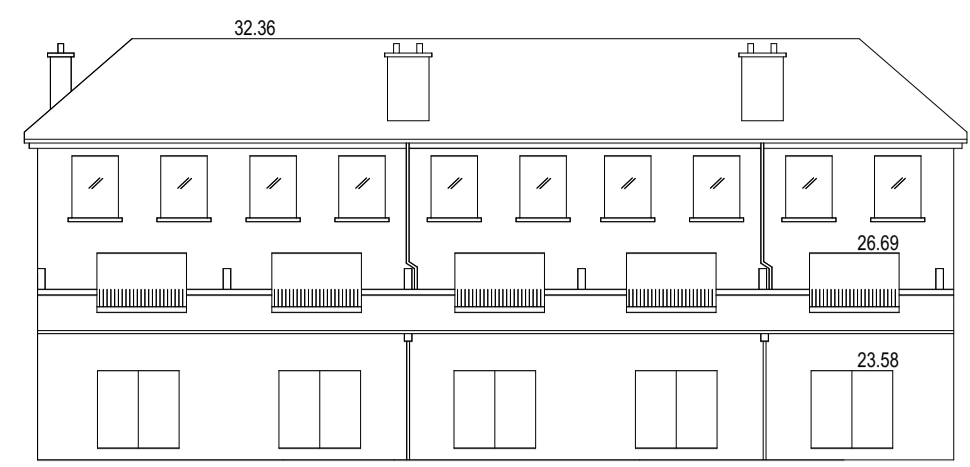
Datum 15.00 AOD Block C East Elevation
