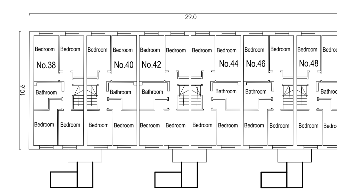
SECOND FLOOR
