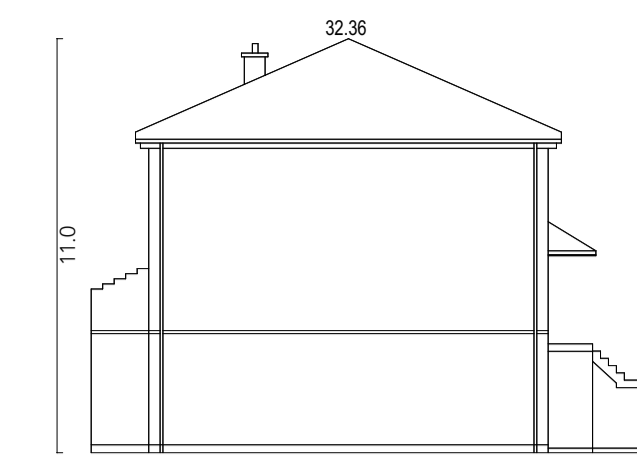
Datum 15.00 AOD Block C North Elevation
