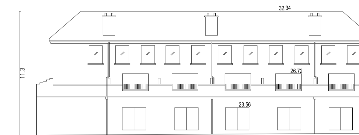
Datum 15.00 AOD Block D East Elevation
