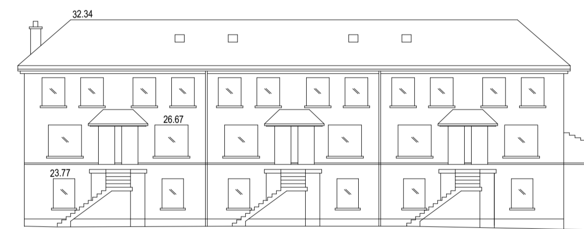
Datum 15.00 AOD Block D West Elevation
